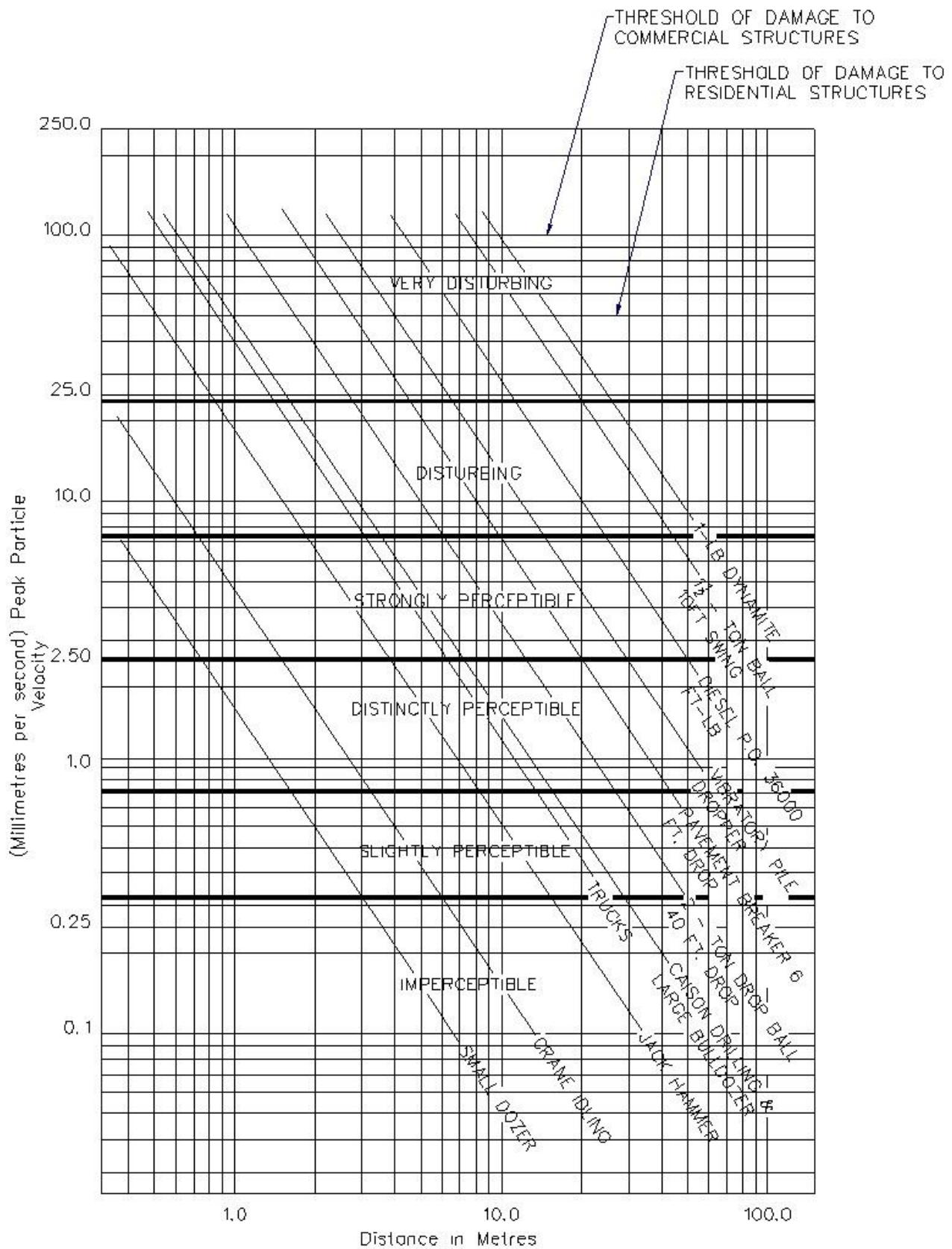
CONSTRUCTION VIBRATION INTENSITIES RELATED TO HUMAN EVALUATION OF VIBRATIONS AND DAMAGE CRITERIA
